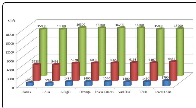
Figure 8. The multiannual average, maximum and minimum flows at main hydrometric stations (1931 – 2020).
