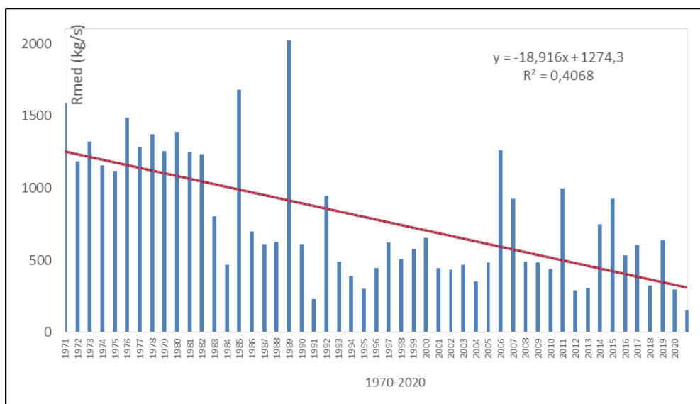
Figure 19 The variation in the suspended solids annual average flow at the Ceatal Chilia hydrometric station (1971-2020)
