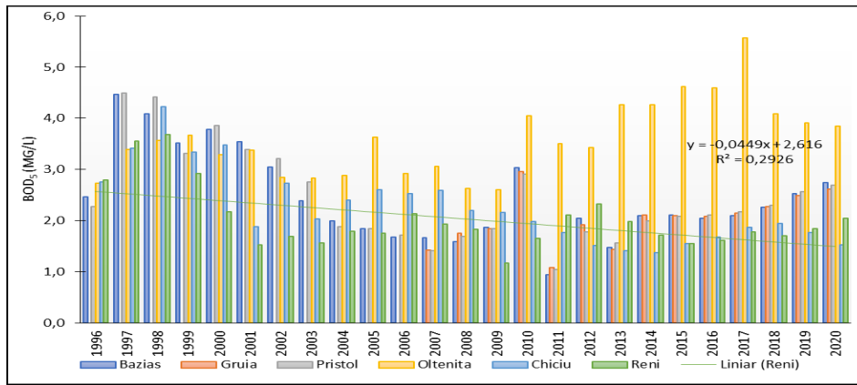
Figure 20. The variation in annual average values of BOD 5 concentrations (1996-2020).
