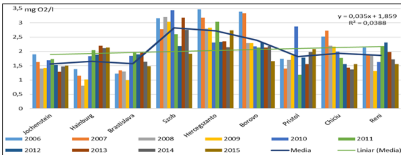
Figure 5. The annual and multi-annual variation in BOD 5 average concentrations (2006-2015) on the Danube River
