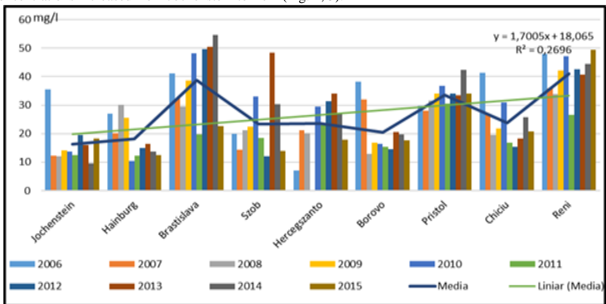
Figure 4. The variation in the annual and multiannual average values (2006-2015) of suspended solids concentrations on the Danube River.
