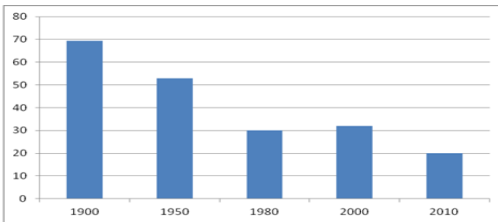
Figure 18. The decrease in the annual flow of suspended sediments at the Isaccea hydrometric station (million t/year) (INHGA).
