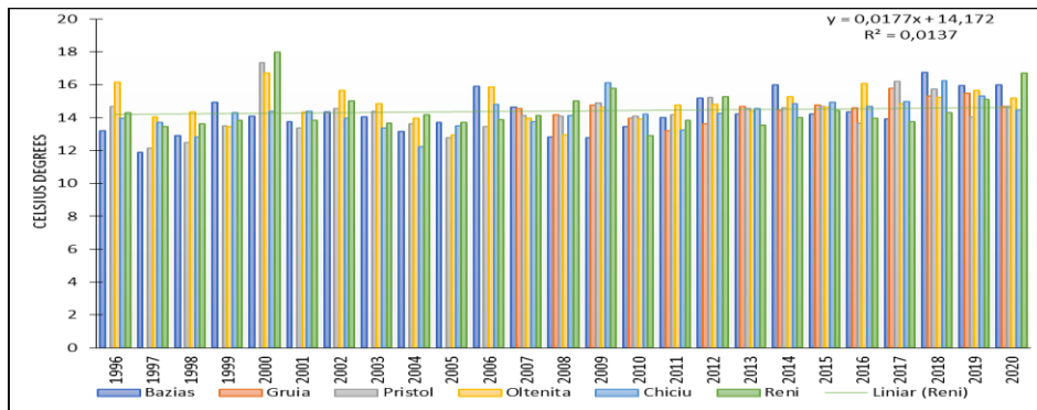
Figure 21. The variation in annual average water temperature (1996-2020).
