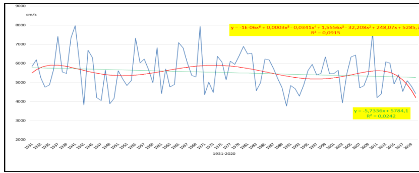
Figure 9. The variation in the annual average flow at Baziaș (1931-2020).
