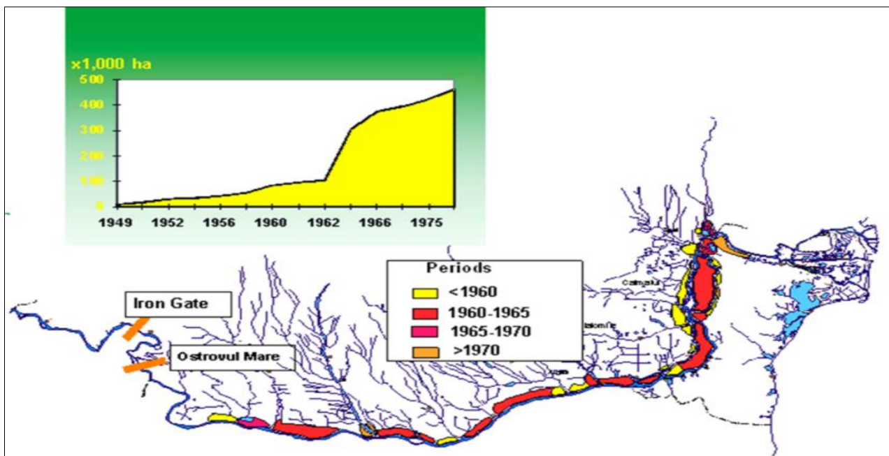
Figure 7. The evolution of the Danube floodplain damming actions (NIRD Delta Dunării).
