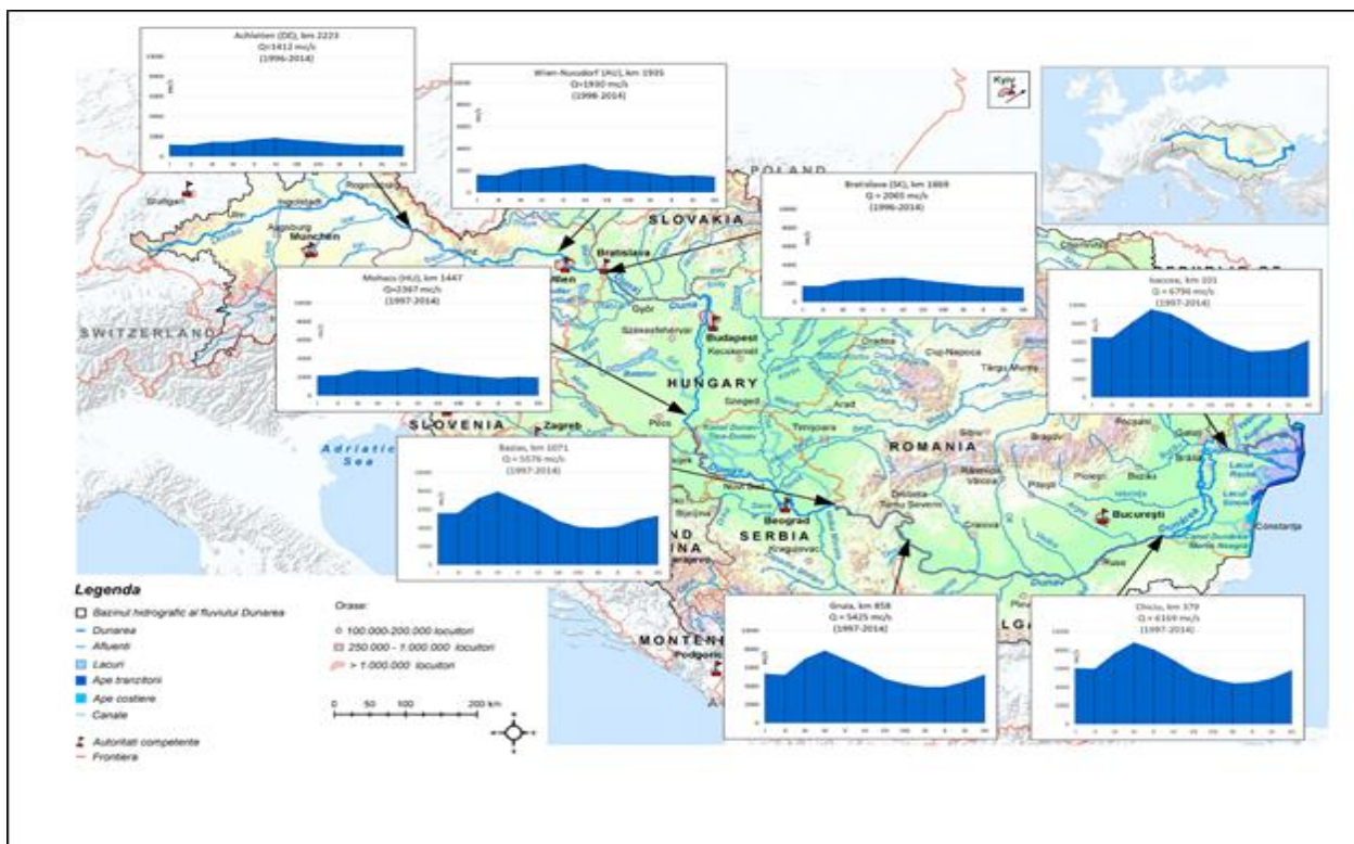
Figure 2. The variation in multiannual monthly average discharges of the Danube River at main hydrometric stations (Țuchiu, 2018).
