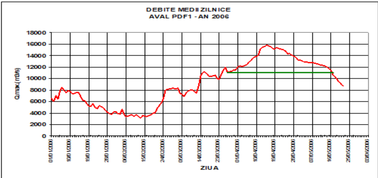
Figure 15. The flow downstream of the Iron Gates during March-May 2006 (Șerban and colab, 2006).
