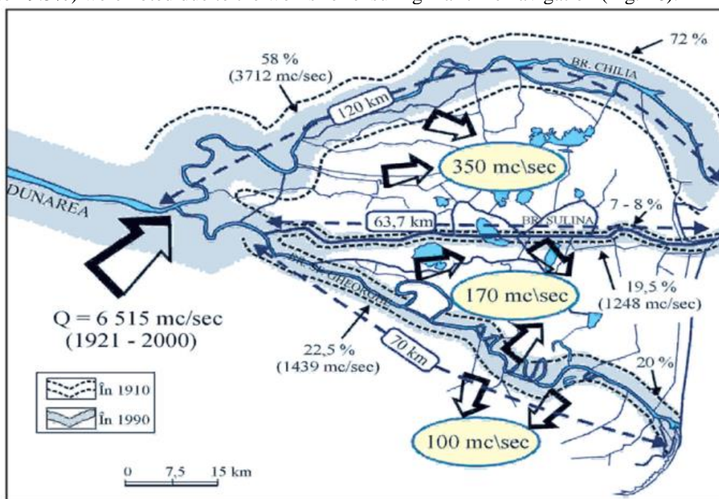
Figure 16. The distribution of water flows on the Chilia, Sulina and Sfântu Gheorghe arms.
