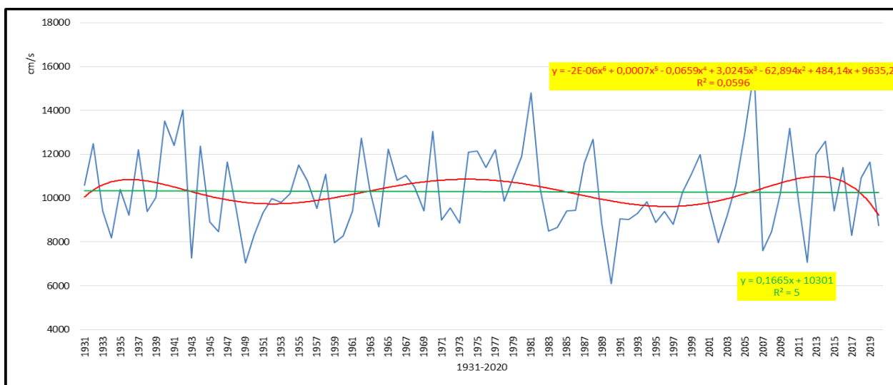
Figure 13. The variation in the annual maximum flow at Baziaș (1931-2020).
