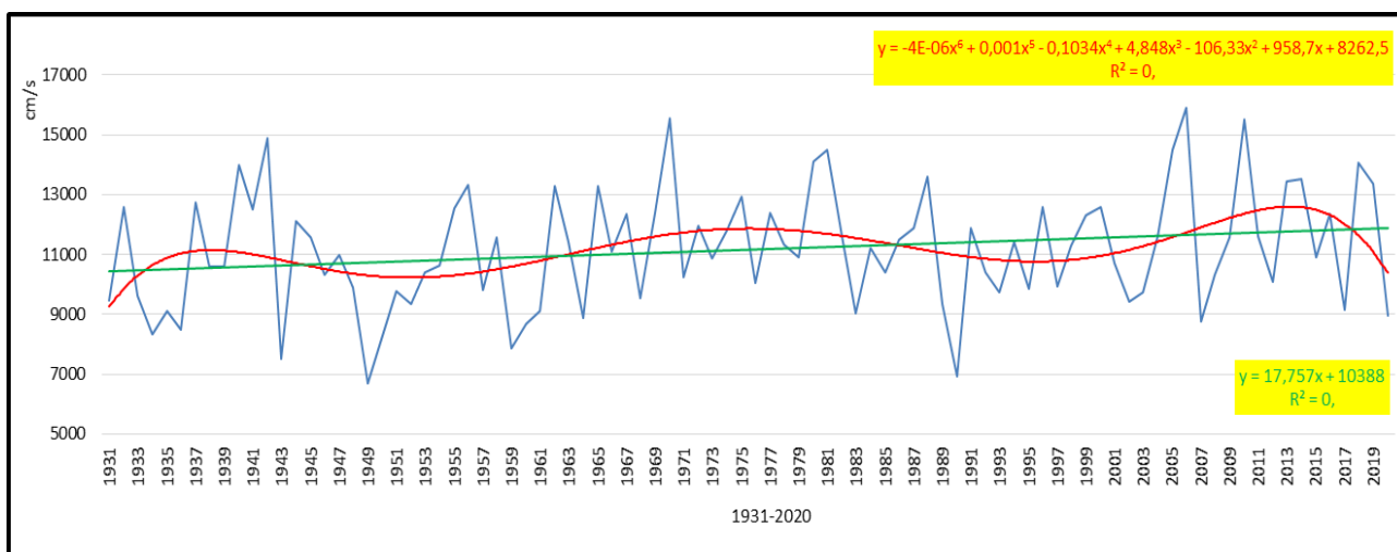
Figure 14. The variation in the annual maximum flow at Ceatal Chilia (1931-2020).
