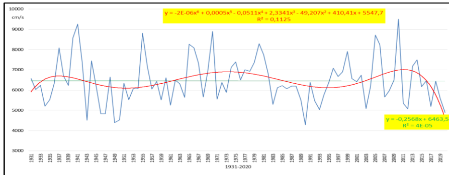
Figure 10. The variation in the annual average flow at Ceatal Chilia (1931-2020).
